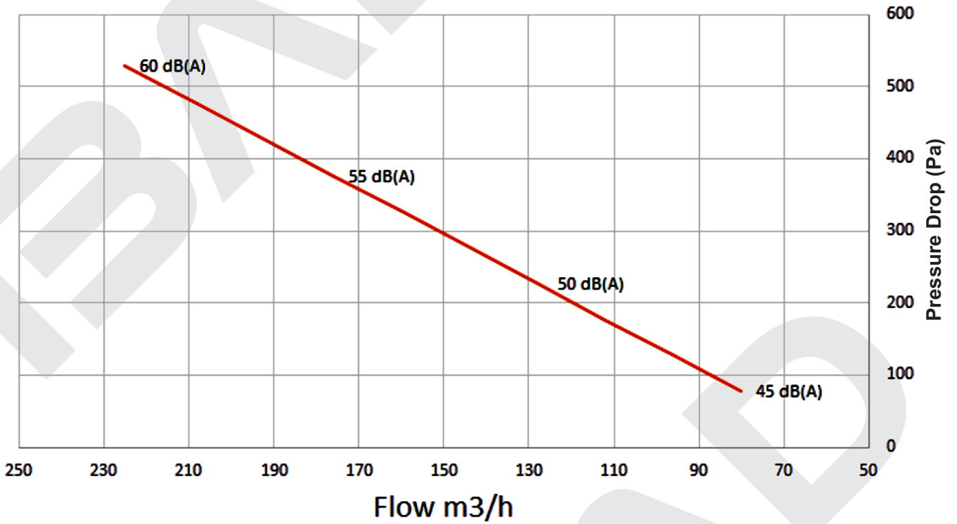
Pressure Drop chart
